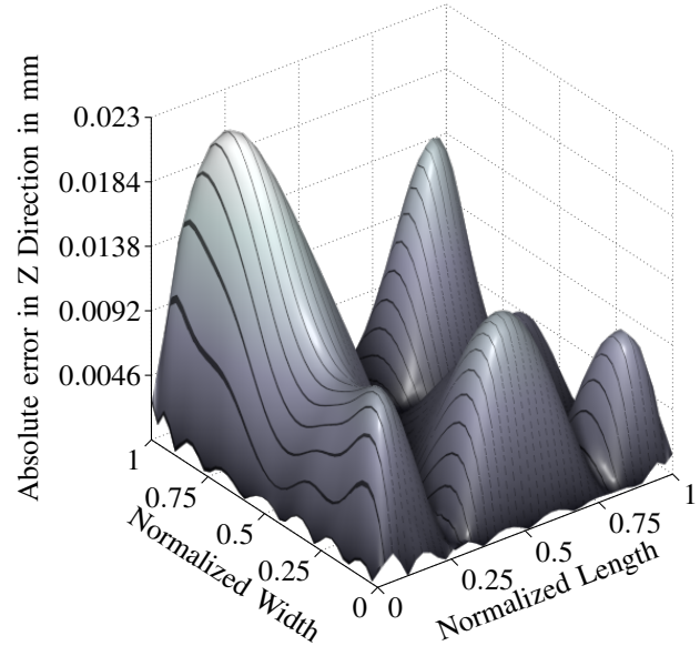
Fig. 6. Distribution of absolute error in z-direction compared to the exact solution for simply supported thin plate under transverse load.
